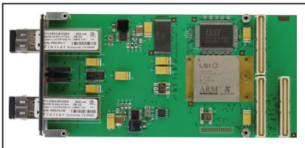
Dual 4 Gbit/s Fibre Channel PMC
