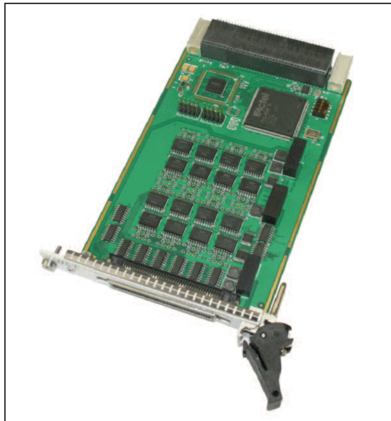
64-Channel Isolated Analog to Digital Converter Board
