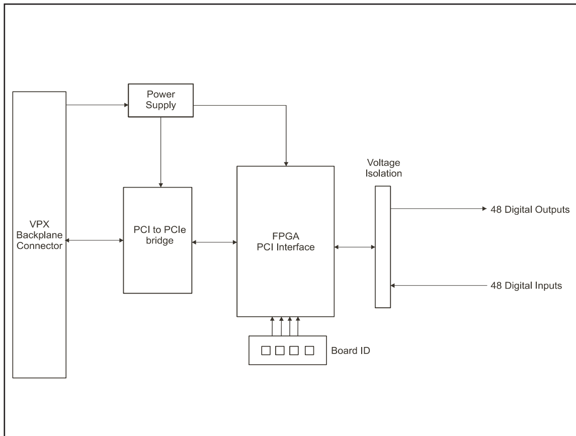
Block Diagram of a 96-Channel Isolated Digital I/O Board
