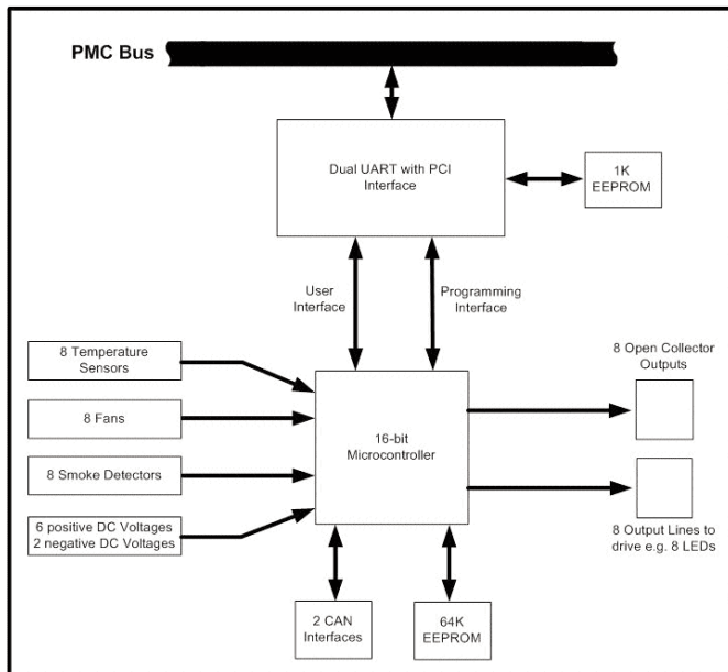
EMAC Architecture
