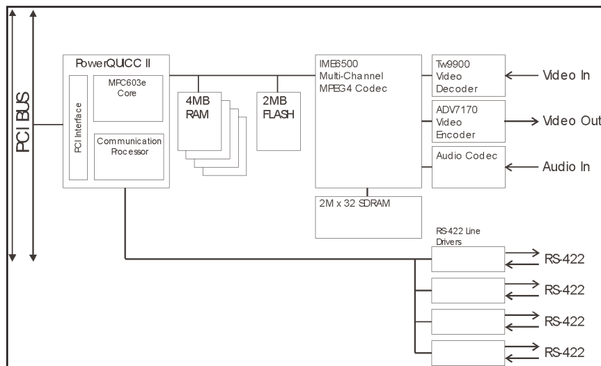
Video Capture and Compression Block Diagram
