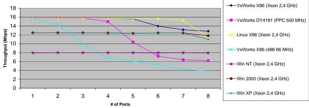
Throughput Values for the HSS8 Adapter (Sending 16 kbyte packets @ 16 Mbps)
